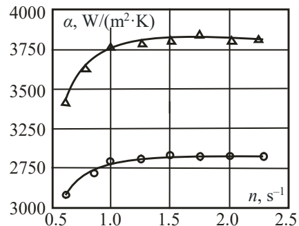
Fig. 3. Dependence of the heat transfer coefficient on the rotor speed: O – with the basic structure of a rectangular blade; \Delta – with an advanced blade equipped with an autonomous system for heating the reflective surface
