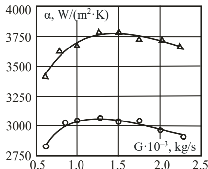
Fig. 2. Dependence of the heat transfer coefficient on the flow rate of the experimental raw material: the O curve for the basic design of the rectangular blade; the \Delta curve for the cutting blade provided with an autonomous system for heating the reflective surface
